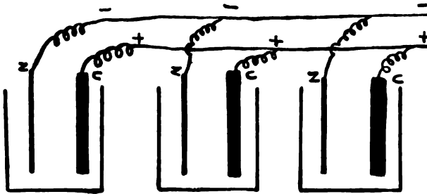
FIG. 423.—Diagram of a Multiple , or Parallel , Circuit, showing Three Galvanic Cells in Battery. In this system of forming the battery there are two main lead wires, one connected to the positive poles of all the cells, the other to the negative poles. Unlike the series system shown above, the effect is that the total voltage of the battery is equivalent to the voltage of one of the cells only, the pressure seemingly being cut down by this wiring. If, on the other hand, a number of motors, or other electrically affected apparatus, be connected in multiple, the "back-pressure" (C. E. M. F.) is similarly decreased, enabling each one to give its highest operative efficiency.
